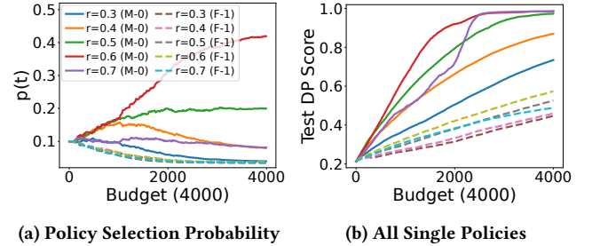
Figure 8: A detailed analysis for Figure 7a. (a) FALCON increases the selection probability of r = 0.6 for the subgroup ( M - 0 ), where we denote the sensitive attribute (Male or Female) and label of the target subgroup in parentheses. (b) Fairness improvements for all single policies. The policy r = 0.6 for ( M - 0 ) is the most effective in improving fairness.
