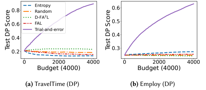
Figure 3: Comparing trial-and-error approach with the baselines on the TravelTime [22] and Employ [22] datasets where the target fairness is demographic parity (DP). Only the trial-and-error solution actually improves the DP score.
