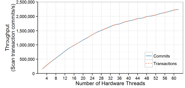
Figure 4: YCSB E scan transaction throughput as the number of client threads is varied.
