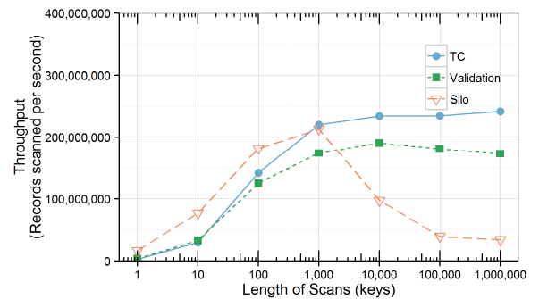
Figure 8: MVCC range scan throughput for various approaches.
