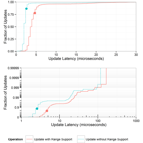
Figure 5: Update operation latency both with and without range support.
