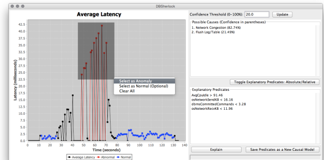
Figure 3: Screenshot of DBSherlock's user interface
