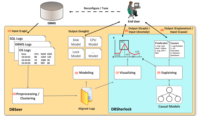
Figure 1: DBSeerArchitecture
