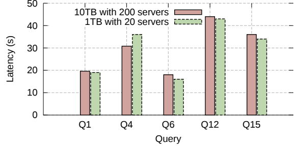
Figure 10: JETSCOPE Scalability.
