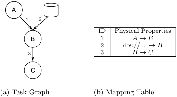
Figure 5: A Channel Abstraction Example.
