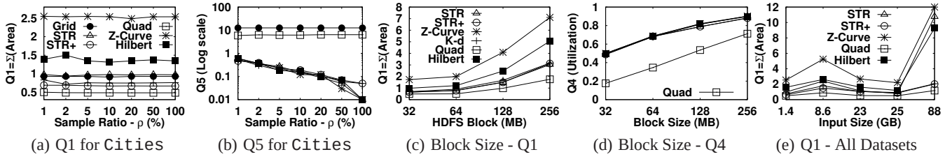
Figure 3: Quality Measures
