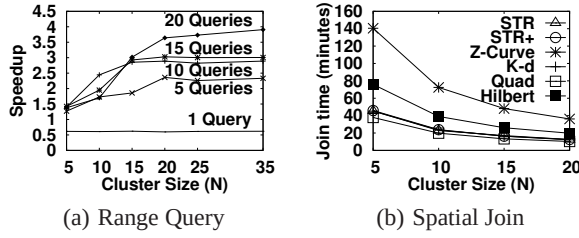
Figure 5: Scale-out with cluster size
