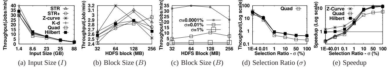
Figure 4: Range Query
