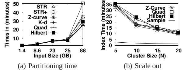
Figure 7: Partitioning Time
