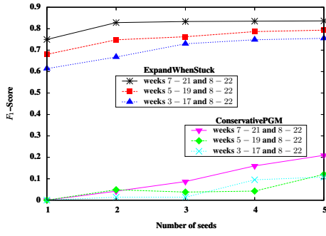
Figure 10: F_1 -score (see Equation (7)) vs. number of seeds. Simulations are done over EPFL e-mail network with. Each snapshot of the e-mail network is created by aggregating all the exchanged e-mails in a given time period.
