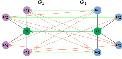
Figure 2: ExpandWhenStuck (Algorithm 3): Nodes u_1, u_2, u_3, u_4 and u_5 are unmatched neighbours of node u in the underlying graph G (see Example 2 and Figure 1).
