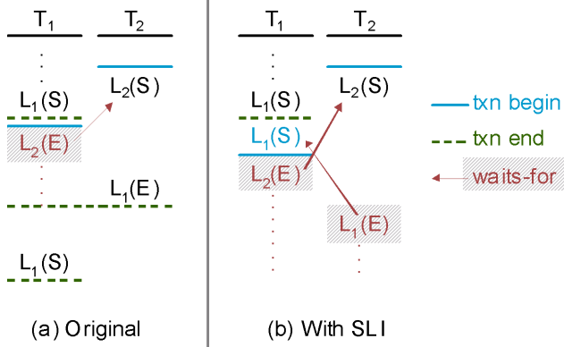
Figure 4. Example of potential SLI-induced deadlock
