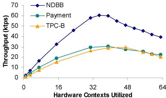
Figure 7. Impact of lock manager bottleneck as load varies.
