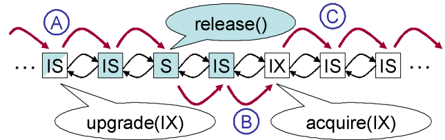
Figure 3. Lock release example
