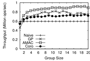
(a) 1 Thread Varying Group Size
