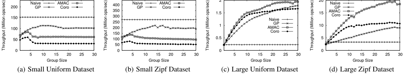
Figure 2: MSVC Hash Index Probe 1 Thread Varying Group Size
