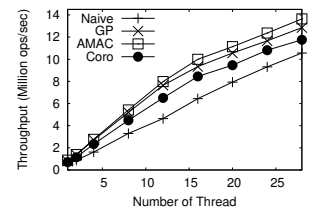
(c) 12 Group Size Varying Thread
