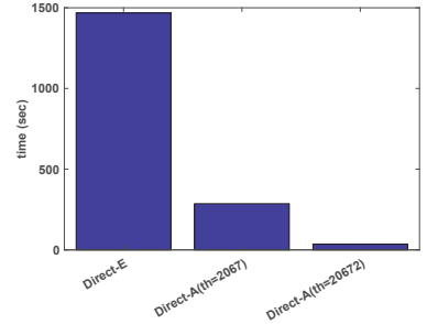
Figure 15: Execution time of DIRECT-E, DIRECT-A ( \tau=2067 ), and DIRECT-A ( \tau=20672 ) in p2p-3
