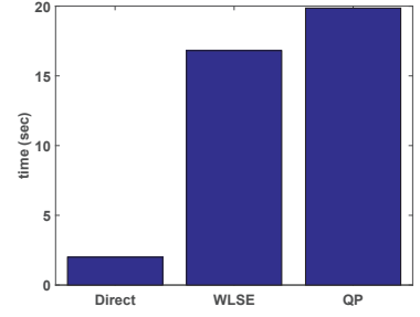
Figure 12: DIRECT v.s. baselines in N_3 : n = 1,421 and m = 21,058
