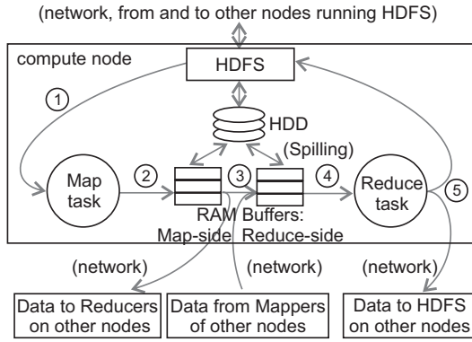
Figure 3: Schematic dataflow between map, reduce, HDFS, RAM, and filesystem in one Hadoop compute node. Dataflow from and to remote map, reduce, and HDFS instances.
