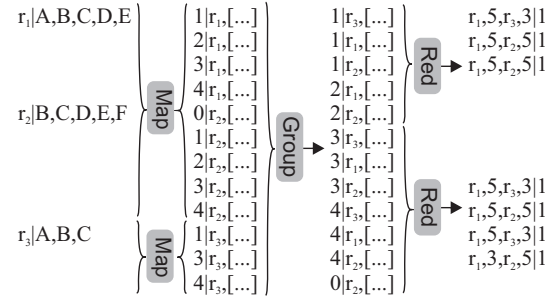
Figure 18: FS-Join, Job 3, Example. Pivots are B,D,E,F.
