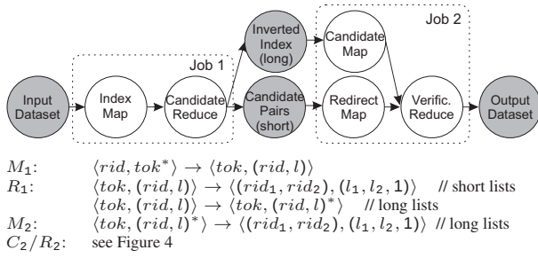
Figure 6: V-SMART Dataflow
