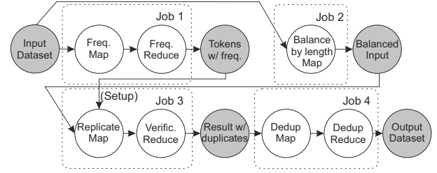
Figure 9: MGJoin Dataflow.
