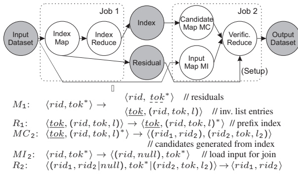
Figure 11: SSJ-2R Dataflow.
