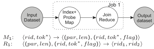
Figure 15: MRGroupJoin Dataflow.
