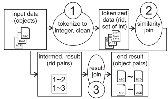
Figure 2: Computation of a token-based SSJ. Our work focused on step (2), the actual join.
