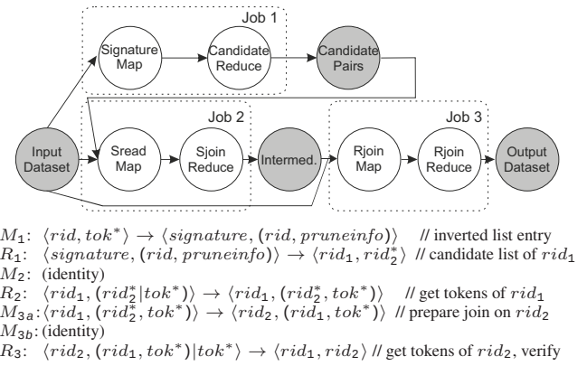
Figure 13: MassJoin Dataflow.
